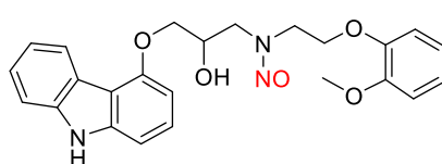
N-nitroso-carvedilol
