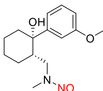
N-nitroso-desmethyl- tramadol
