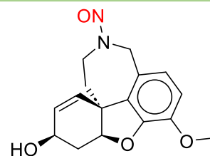
N-nitroso-desmethyl-Galantamine
