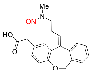
N-nitroso-N-desmethylolopatadine
