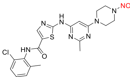
N-deshydroxyethyl-N-nitroso dasatinib
