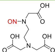
N-nitroso-ethylenediamine-triacetic acid
