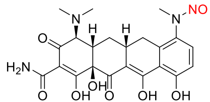
N-nitroso-desmethyl-minocycline Impurity 2
