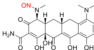
N-nitroso-desmethyl-minocycline Impurity 1
