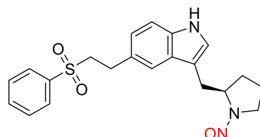
N-nitroso-desmethyl-Eletriptan
