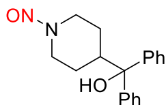
(1-Nitrosopiperidin-4-yl) diphenylmethanol
