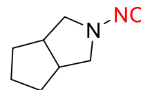
Octahydro-2-nitroso cyclopenta[c]pyrrole
