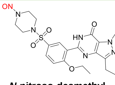
N-nitroso-desmethyl- sildenafil
