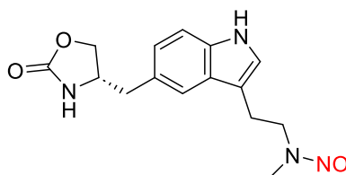
N-nitroso-desmethyl- zolmitriptan
