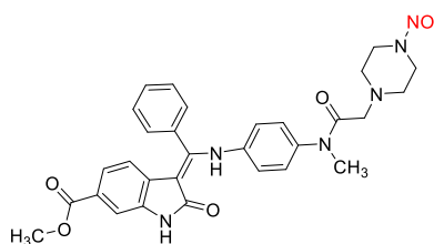
N-nitroso-desmethyl-nintedanib
