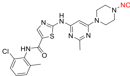
N-deshydroxyethyl-N-nitroso dasatinib
