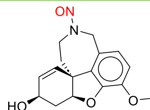
N-nitroso-desmethyl-Galantamine
