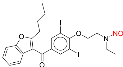
N-Nitroso-desethyl-amiodarone
